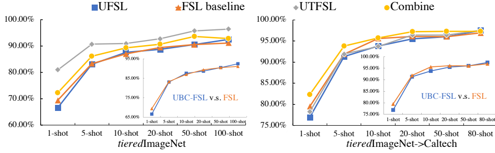
Figure 5: Few-shot classification accuracy with larger shots. We use ResNet-50 as our backbone architecture and evaluate on tieredImageNet and Caltech (transferred from tieredImageNet ).
