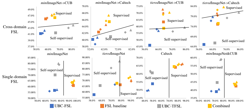
Figure 4: Accuracy of 1-shot cross-domain FSL (first row) or single-domain FSL (second row). First row: we visualize 1-shot test accuracy on the source dataset (x-axis) and the target dataset (y-axis). Second row: we visualize 1-shot accuracy on base categories (x-axis) and novel categories (y-axis). Squares, diamonds, and triangles denote ResNet-12, ResNet-50, and ResNet-101 respectively. Please refer to Table A2, A3 for detailed statistics.
