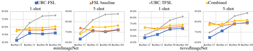
Figure 3: Few-shot classification accuracy with various depths of backbone architectures.
