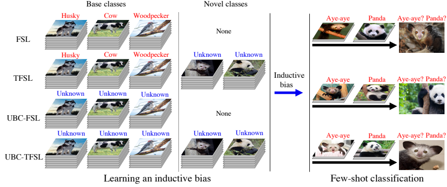
Figure 1: An illustration of different few-shot learning settings. The difference between these settings is whether they have labels for examples from base classes and unlabeled examples from novel classes.
